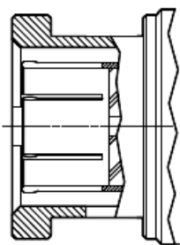
Section A'-A' 75 ohm
